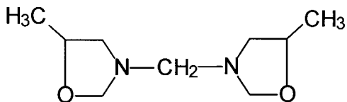
3,3'-Methylen-bis[5-methyl-oxazolidin]
